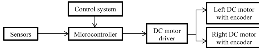
Fig. 1. Two-wheel self-balancing robot construction.
